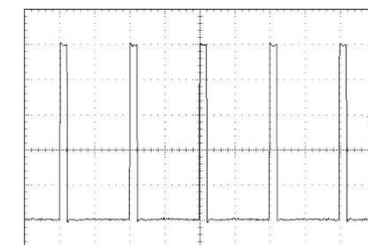
10KHz Repetition Frequency, 6000V Output (50µs/Div horizontal scale, 1.2kV/Div vertical scale)
