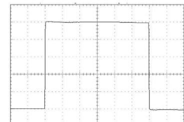
Typical Output Waveform, 6000V Output (25µs/Div horizontal scale, 1.2kV/Div vertical scale)
