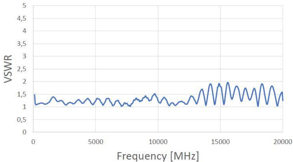
Figure 7: Typical VSWR (845-20)
