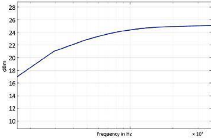
Figure 1: Typical Maximum Output Power from 9 kHz to 1 MHz (options 9)
