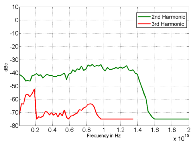
Figure 14: 845-26 with option FILT
