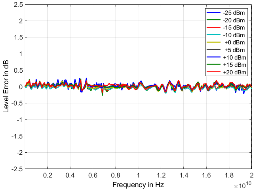
Figure 9: Typical Frequency Response 0 to 20 GHz at -20, 0, and +20
