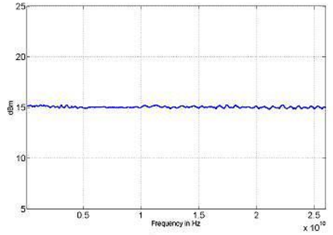
Figure 4: Typical Maximum Output Power 845-20-HP-PE3
