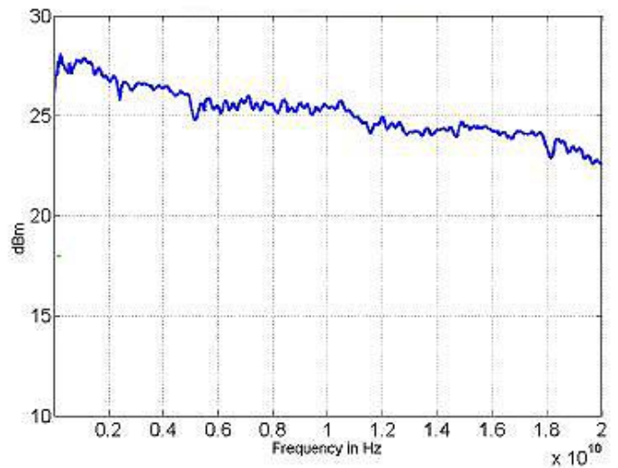
Figure 6: 845-20-HP-PE2
