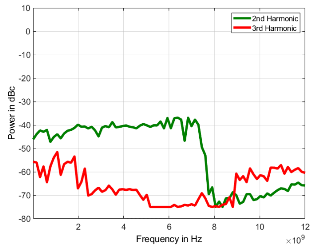
Figure 12: Harmonics 845-12 with option FILT
