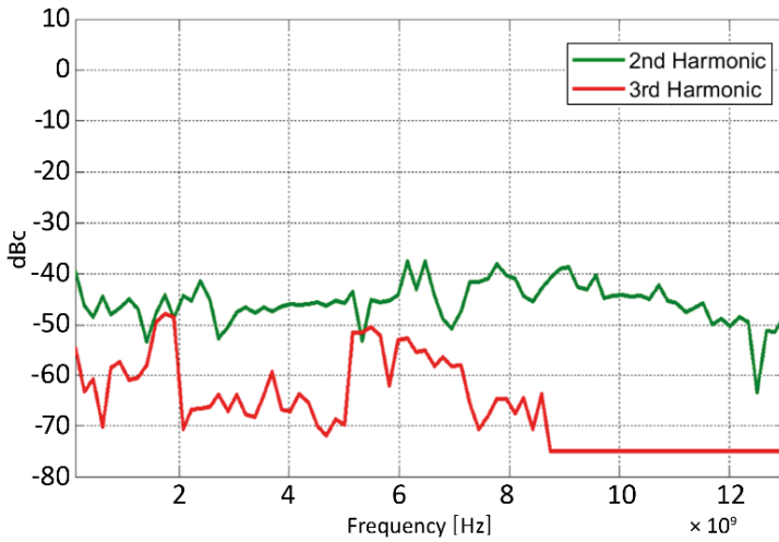
Figure 11: Harmonics Standard
