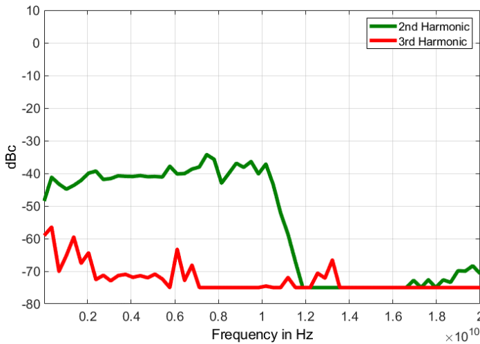
Figure 13: Harmonics 845-20 with option FILT
