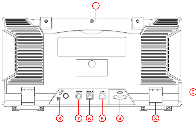
Figure 3-6 Rear Panel
