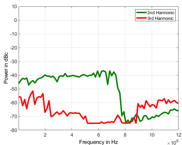
Figure 8: Harmonics 845-12 with option FILT
