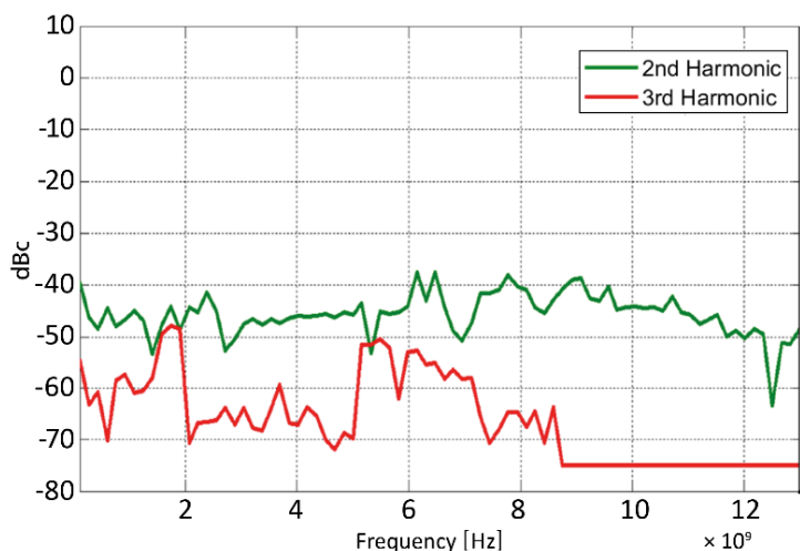
Figure 7: Harmonics Standard
