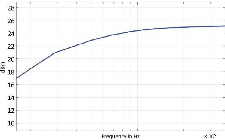
Figure 2: Maximum Output Power 845-26, HP with and without option PE2
